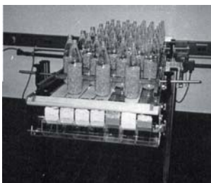
Test station
